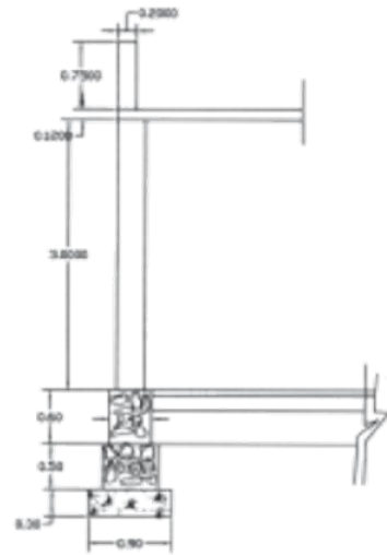
cross section at X-X
